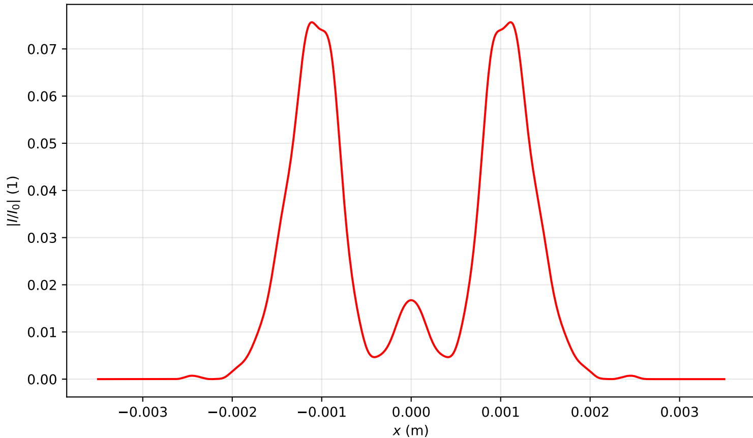
Intensity profile I(x, y = 0, z = 3.105)/I_0 , P_{in}=7.0P_{cr} , artificial time
